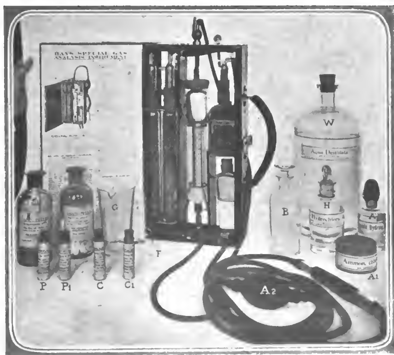
Fig. 3—Line-up of apparatus and chemicals for analysis. Preparations might look tremendous, but the operations are simpler than they seem. Besides muriatic acid and aqua destillata, only caustic potash comes into play when carbon dioxide is to be determined.
